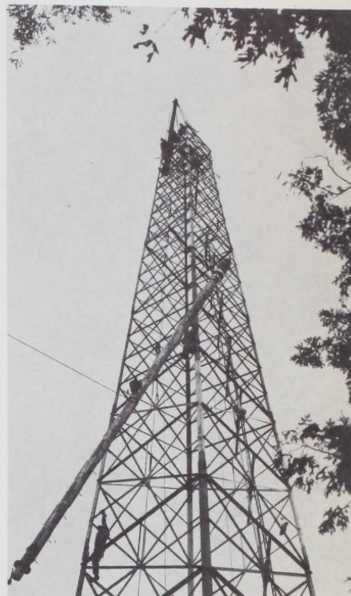
New antenna is shown being lifted to top of 210 foot tower during construction of transmitting equipment on Council Crest. Antenna is made of steel pipe and is 41-feet-long.
