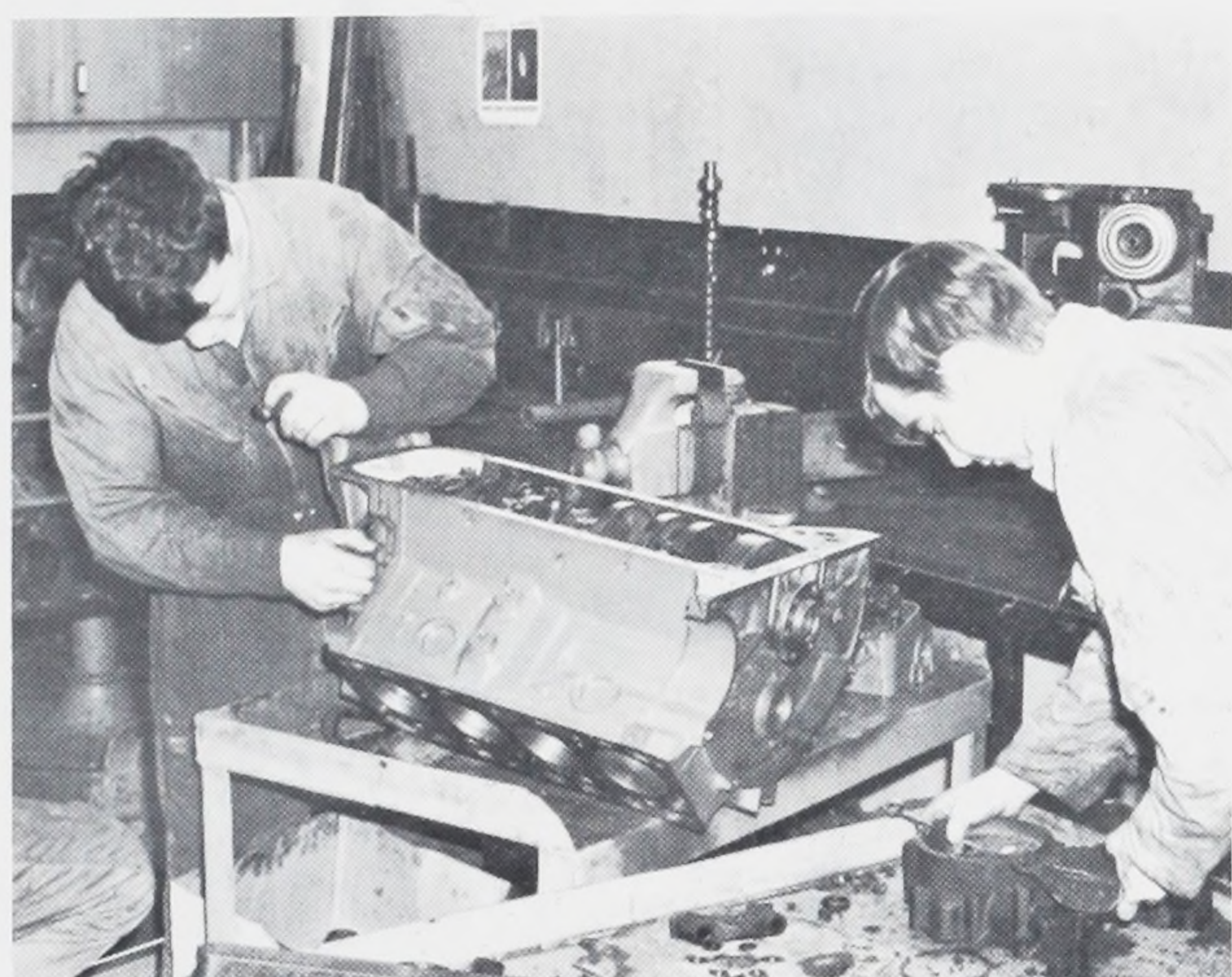
Dale Hochstettler works on his Ford's 312 cubic-inch engine, while Rick Glover repairs his water pump.
