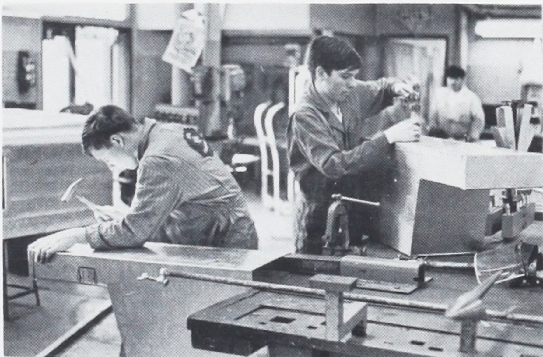
Seniors Bryan Wallace and Bill Herr making gas tanks for pick-up
