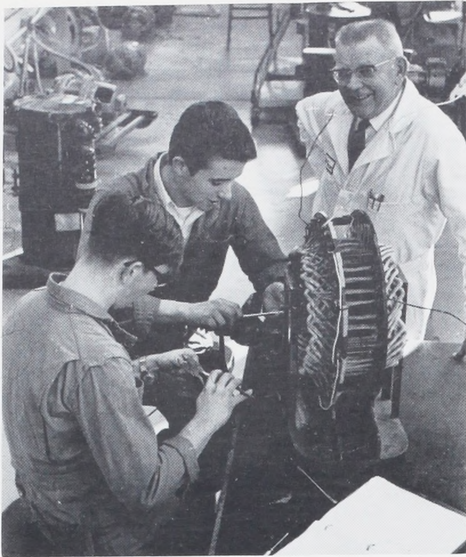
Mr. Lloyd Hanson, Electric Foreman, oversees two of his students working on a three phase A.C. induction motor.
