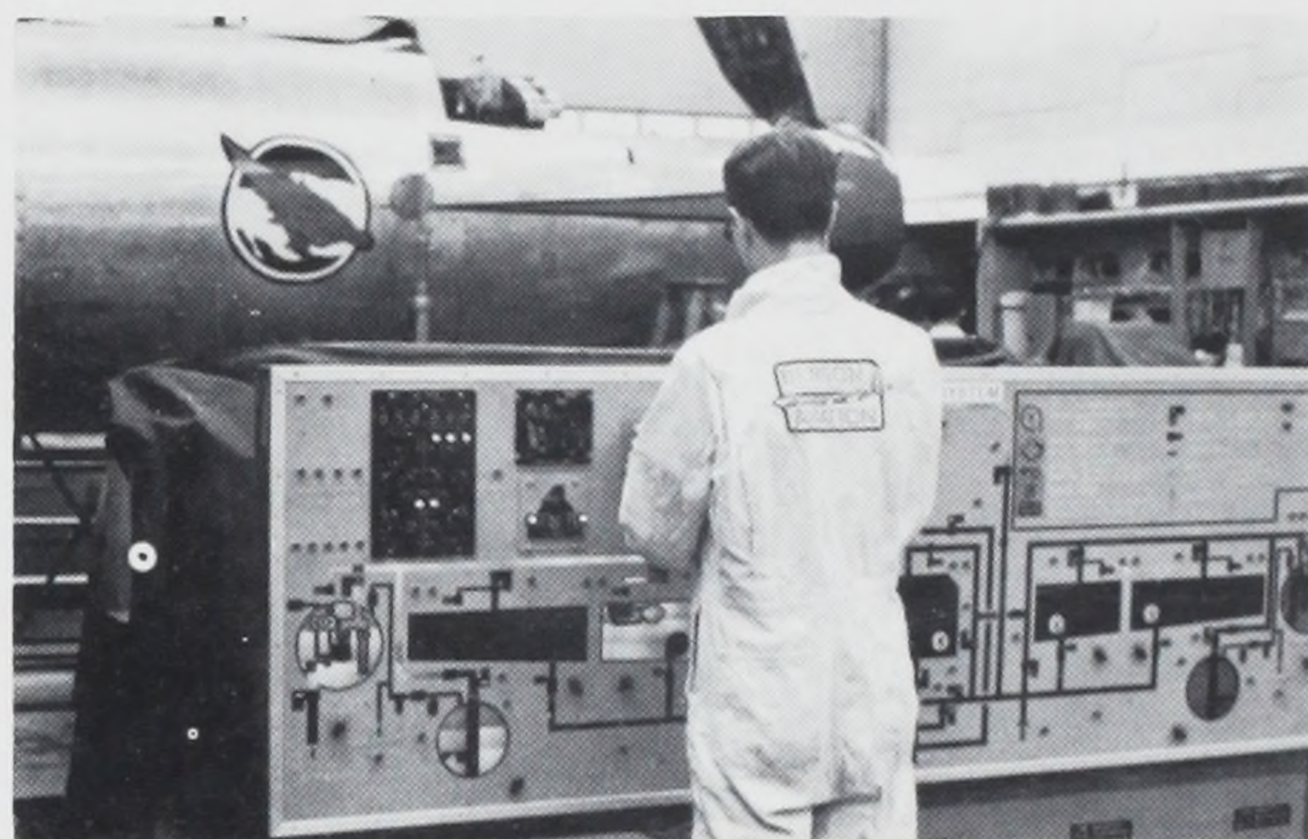
Oscar Wikander works on chart showing complete fuel system of TFEF 89 D/J. Front of F 109 is in background.
